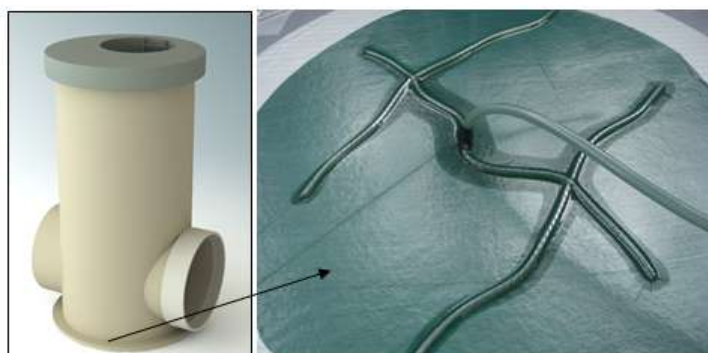
Fig. 1. Base Plate (part of Shaft) manufactured with BIO-UPR by vacuum infusion
