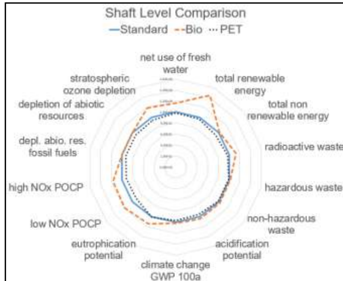
Fig. 4. Shaft Level Comparison
